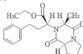
〔2〕 diketopiperazine derivative
